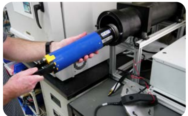
Factory pressure chamber tests leak resistance up to 250m simulated depth
