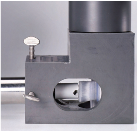
Side view of the YSI 5567 wiper/stirrer assembly with 5561 dissolved oxygen probe attached. The wiper runs continuously utilizing two brushes and providing sufficient stirring to maintain accurate DO data.
