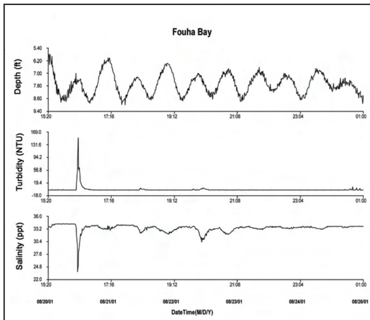
Figure 1. Effect of a short period of rainfall on salinity and turbidity in Fouha Bay, Guam.
