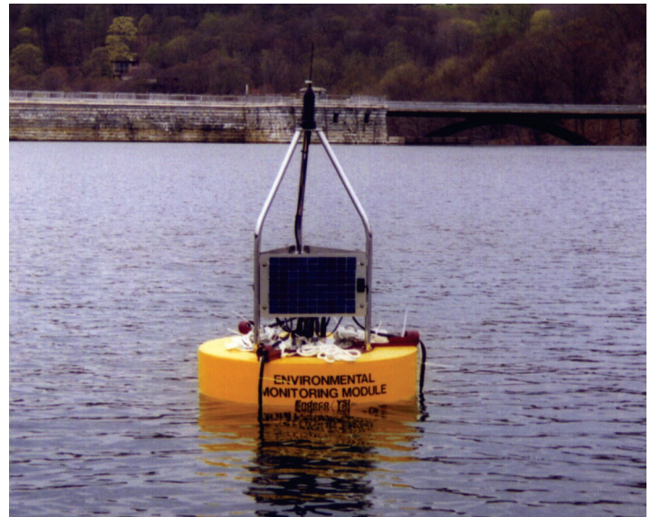
YSI EMM550 Buoy equipped with YSI 6820 sonde and 6200DAS.
