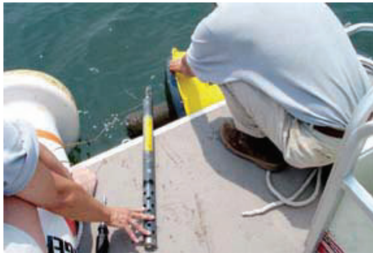
YSI 600OMS and deployment buoy being retrieved by the Reynolds Plantation monitoring crew.
